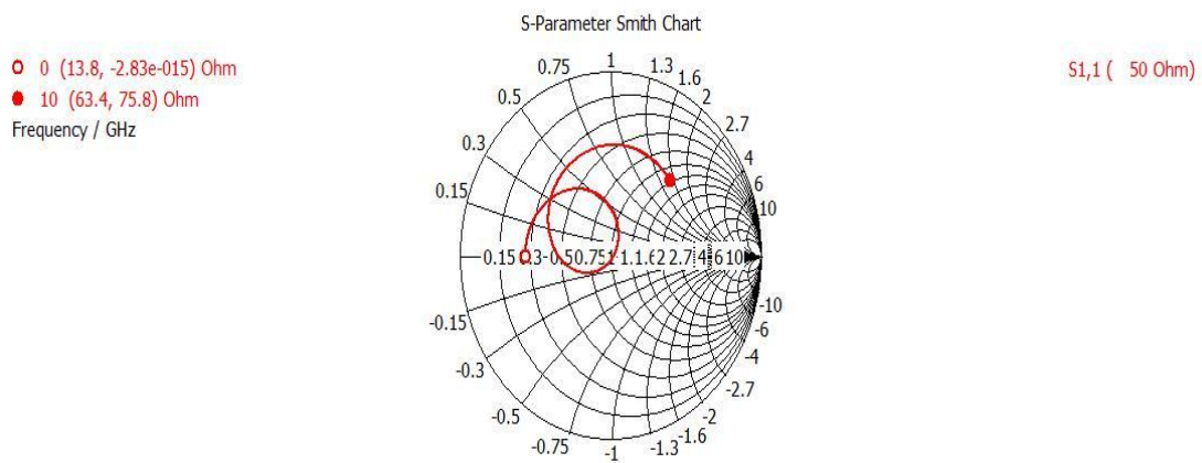
Fig. 5 Characteristic Impedance Curve
