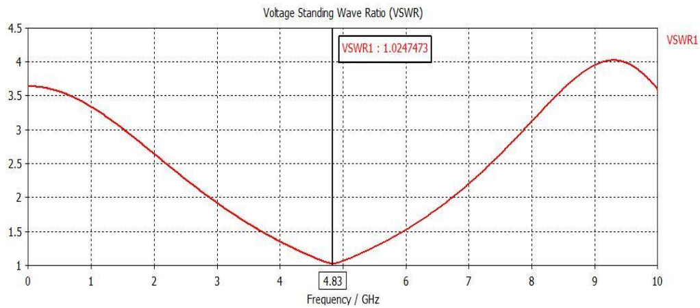
Fig. 6 VSWR Curve
