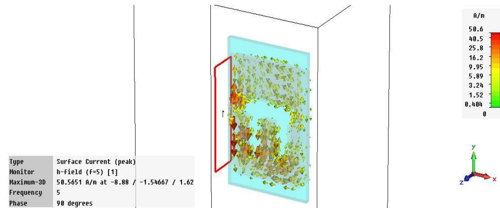
Fig. 7 Surface Current
