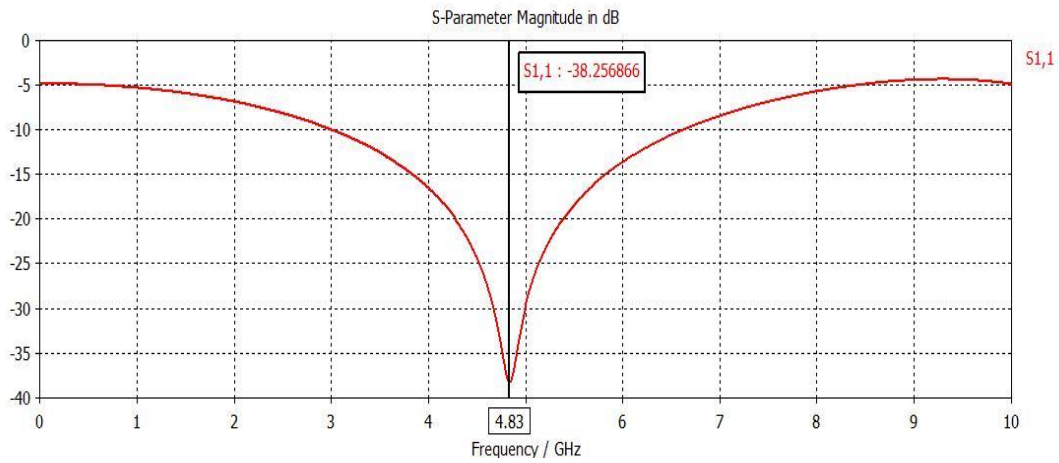
Fig. 4 Return Loss Curve
