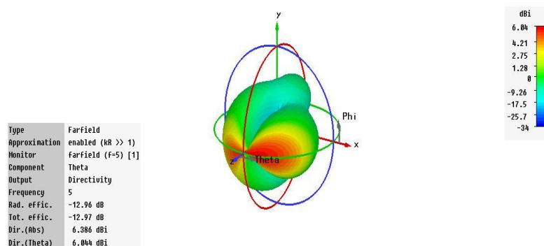
Fig. 8 Directivity Plot
