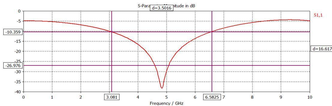
Fig. 3 Bandwidth Plot
