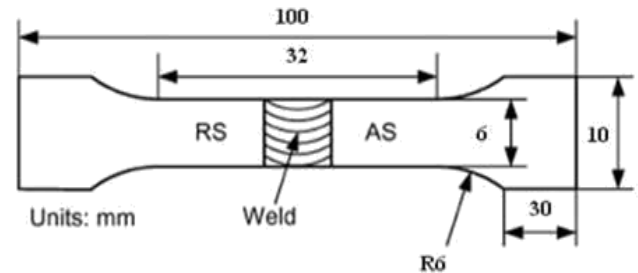
Figure 7. Dimensions of tensile specimen as per ASTM E8 Standard
