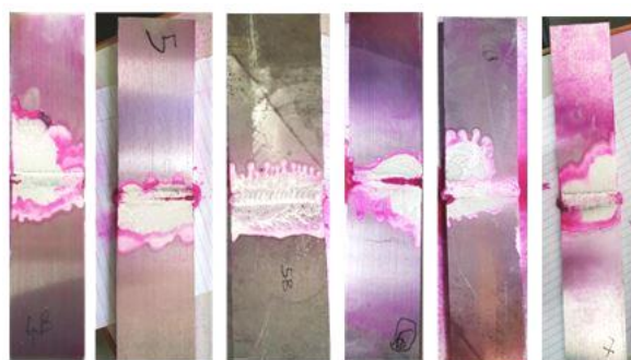
Figure 4. Dye penetrant test samples 1
