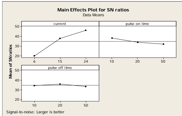
Fig. 5.2: Main effect plot of S/N ratio for MRR.
