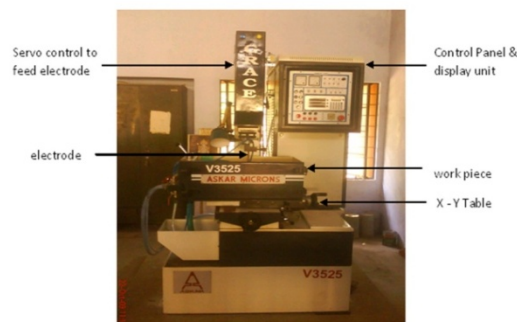
Fig. 1: The Experimental equipment.
