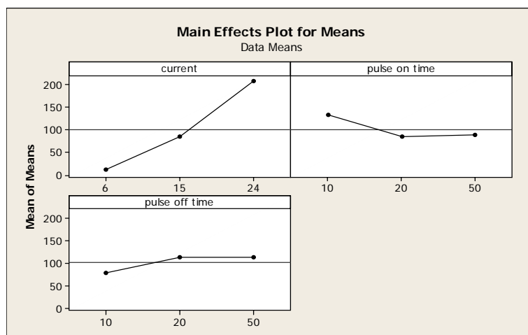
Fig. 5.1: Main effect plot of mean value for MRR.
