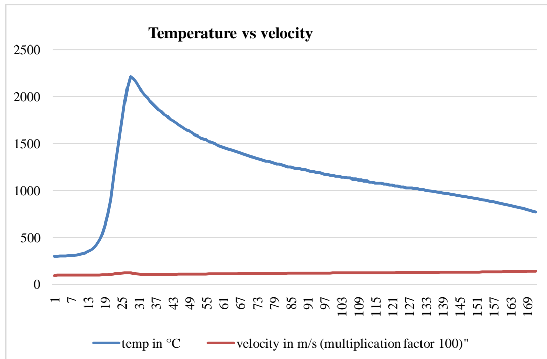
Fig. 6: Temperature vs Velocity chart.
