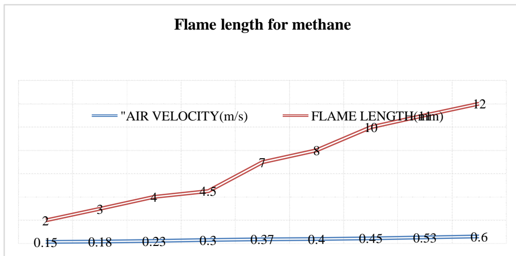
Fig. 4: Air velocity vs Flame length chart.
