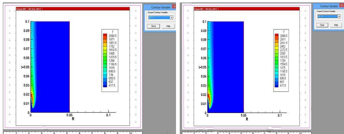
Fig. 1: Flame configuration at 21% oxygen.
