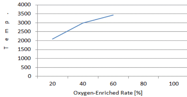
Fig. 3: Temperature vs Oxygen enrichment rate.
