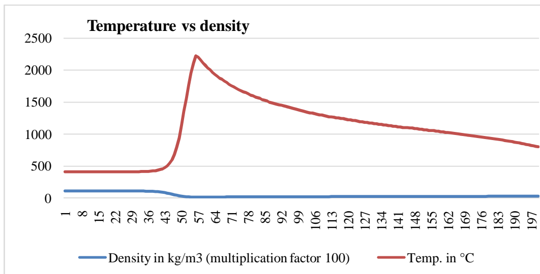
Fig. 5: Temperature vs Density chart.
