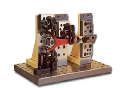
Fig. 1: Modular Fixture[1]
