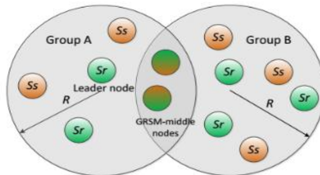
Fig. 2. Group send-recv and GSRM-middle nodes
