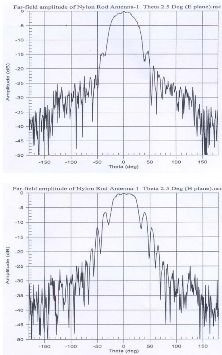
Figure 3: Principle plane patterns of Tapered Nylon rod antenna ( \theta_0 = 2.5^\circ ).
