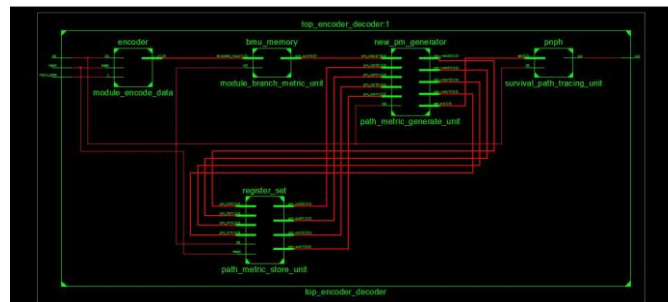
Fig 6:Encoder_Decoder(RTL2)
