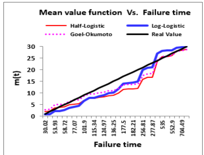
Fig. 4. Pattern of Mean Value Function m(t)
