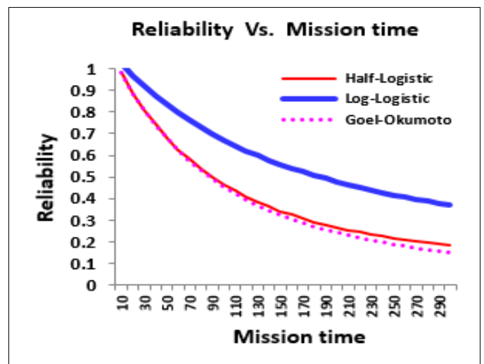
Fig. 5. Transition of Reliability \hat{R}(t)
