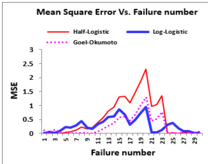
Fig. 2. Transition of Mean Square Error
