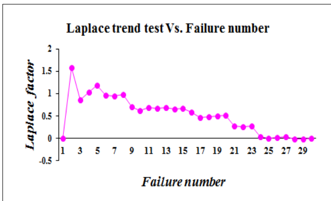
Fig. 1. Estimation Results of Laplace Trend Test
