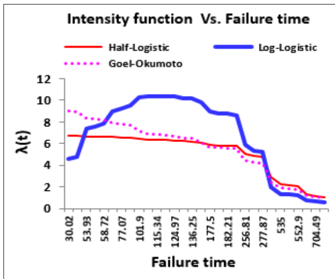
Fig. 3. Transition of Intensity Function \lambda(t)
