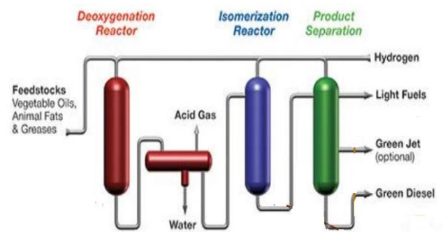
Fig. 2. Production process of green diesel [57]
