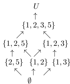
mL(U, A, F) , where A = \{a, b, c, d, e\}
