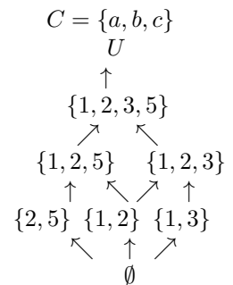
mL(U, C, F_C)
