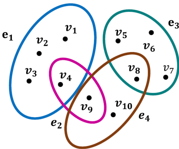
Fig. 1: Hypergraph structure
