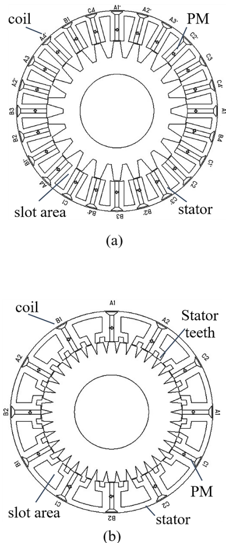
Fig. 1. Cross-section of conventional and proposed SFPM generator; (a) 24/22-pole multi-phase structure with 12-phases and (b) 12/38-pole multi-tooth with 6-phases.
