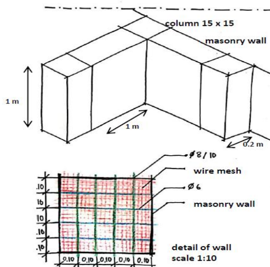
AXONOMETRIC SIMPLE SHEAR WALL SECTION SCALE 1:10
