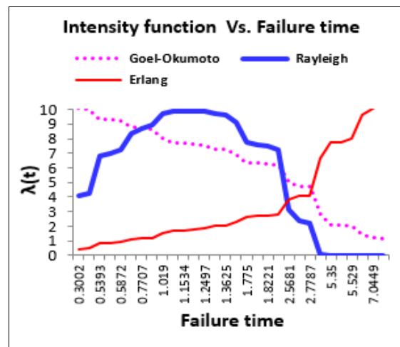
Fig 3. Transition of Intensity Function \lambda(t)
