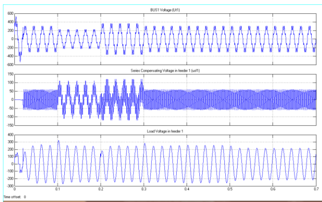
Fig.7 simulated results for bus1 voltage, its series compensating voltage and load voltage in Feeder 1
