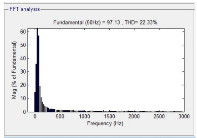
Fig.14 THD for utility side current without MC-UPQC
