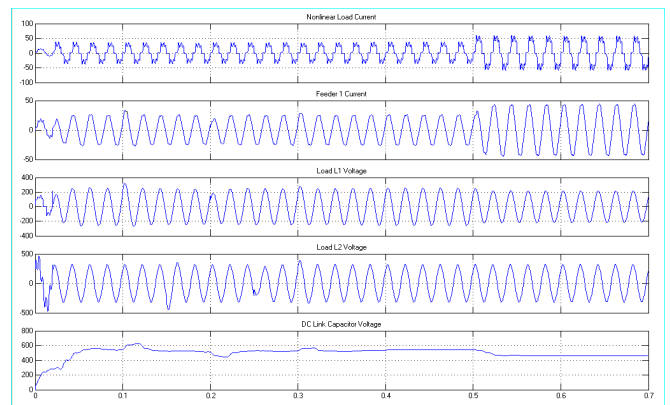
Fig. 10 Simulation results: Nonlinear load current, Feeder1 current, load L1, L2 voltages and DC-link capacitor voltage for load change with PI controller.
