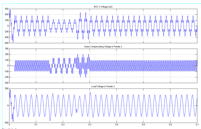
Fig. 8 Simulated results for BUS2 voltage, series compensating voltage in feeder 2, and its load voltage.
