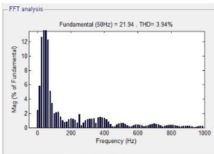
Fig.18 THD for utility side current with FUZZY controller using MC-UPQC (with d-q method)
