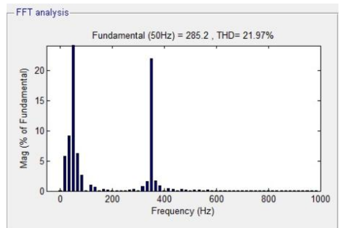
Fig.15 THD for utility side voltage using PI controller with MC-UPQC (with d-q method).
