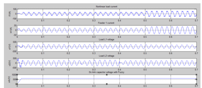
Fig. 11 Simulation results for: Nonlinear load current, Feeder1 current, load L1, L2 voltages and DC-link capacitor voltage when load change with FUZZY controller.
