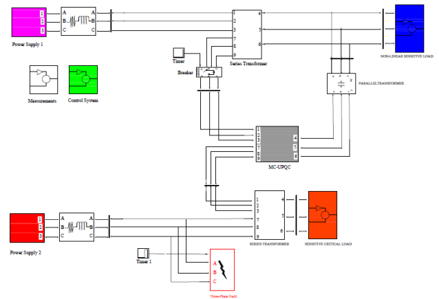
Fig.2 Typical Sim-link Block diagram MC-UPQC used in distribution system
