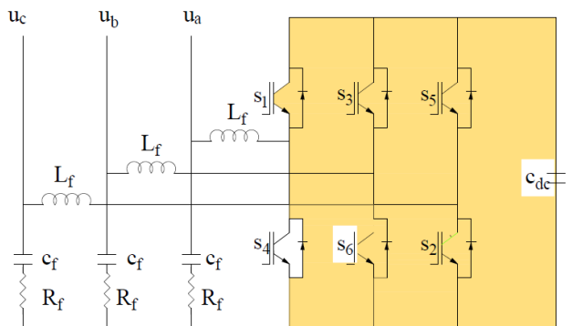
Fig.3 Schematic structure of a VSC
