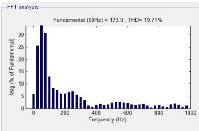
Fig.17 THD for utility side voltage with FUZZY controller using MC-UPQC (with d-q method)
