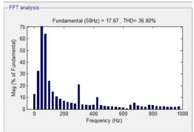
Fig. 13 THD for utility side voltage without MC-UPQC
