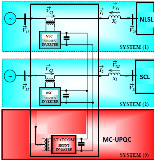
Fig.1. Block diagram of MC_UPQC with STATCOM
