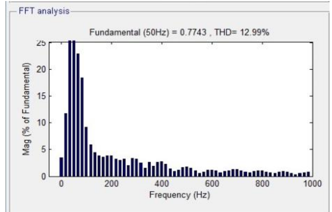
Fig.19 THD for utility side voltage using NEURO-FUZZY controller with MC-UPQC (with d-q method)
