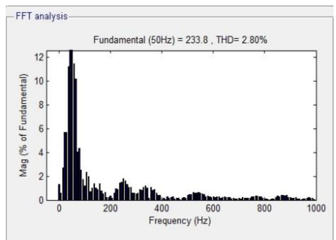
Fig.20 THD for utility side current using NEURO-FUZZY controller with MC-UPQC (with d-q method).
