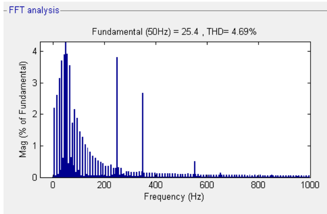
Fig.16 THD for utility side current using PI controller with MC-UPQC (with d-q method)
