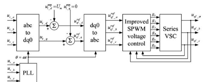
Fig.5. Control block diagram of the series VSC
