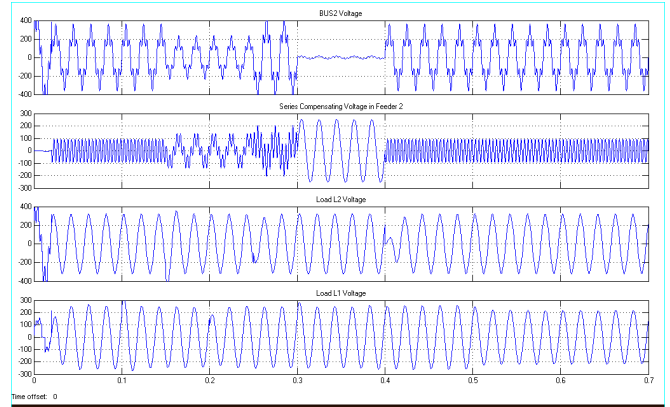
Fig. 9 simulated results for BUS2 Voltage under fault condition, its Series compensation Voltage in feeder 2.
