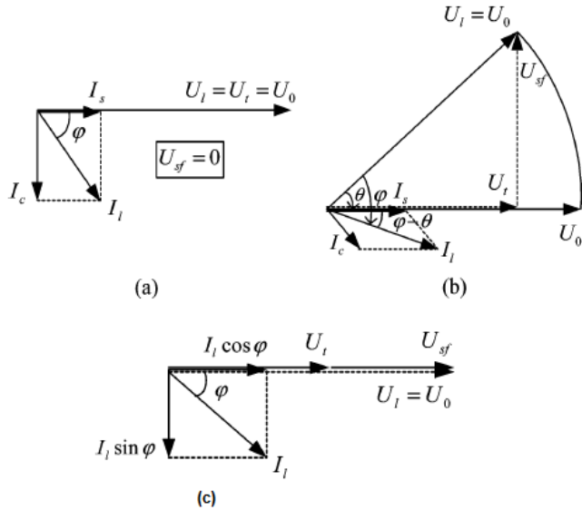
Fig.6. phasor diagram of quadrature compensation. (a)Without voltage sag. (b)With voltage sag.(c) phasor diagram of in phase compensation(supply voltage sag)
