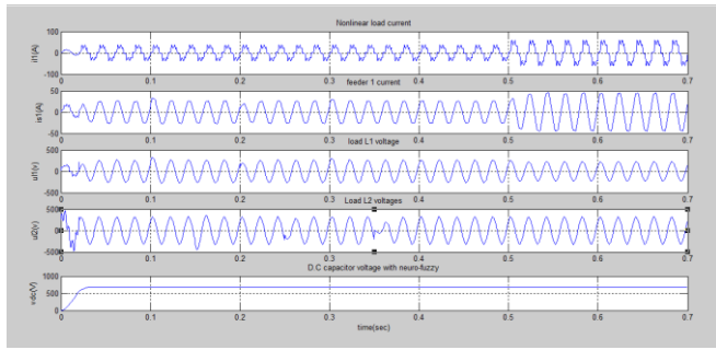
Fig.12.Simulation results: Nonlinear load current, Feeder1 current, load L1, L2 voltage and DC-link capacitor voltage for load change with NEURO-FUZZY controller.
