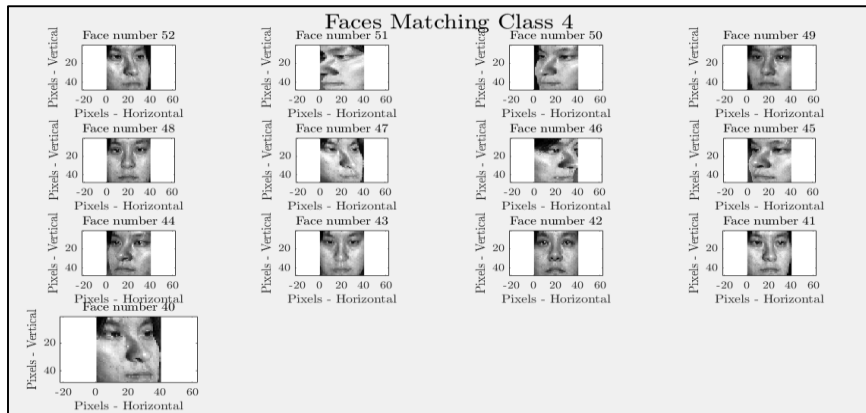
Figure 3.8 Dataset Class 4
