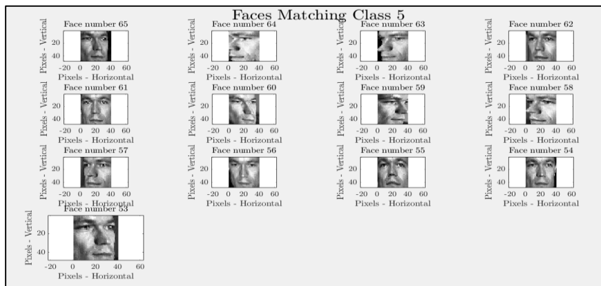
Figure 3.9 Dataset Class 5
