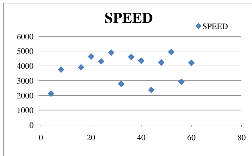
Fig. 3: TIME (in minutes) vs. RPM of alternator.
