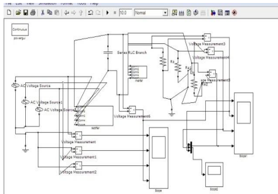
Fig 1: Simulation model of static UPS
