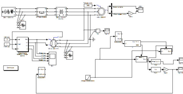
Fig 2: simulation model of rotary UPS without Flywheel
