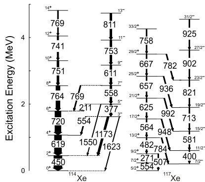
Figure 4. Partial level schemes of ^{114}\text{Xe} and ^{117}\text{Xe} .
