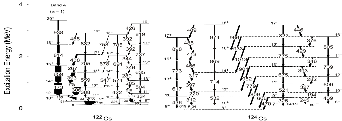
Figure 2. Partial level schemes of ^{122}\text{Cs} and ^{124}\text{Cs} .
