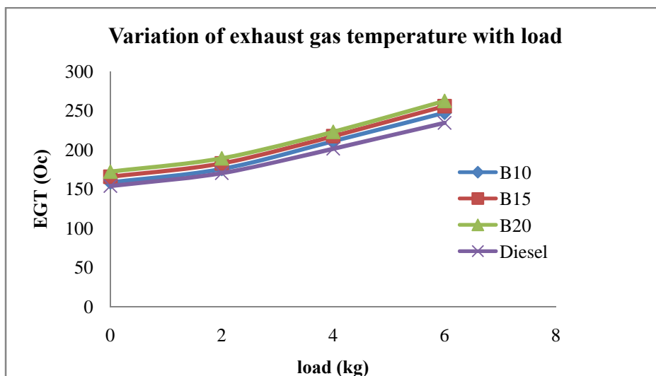
Fig. 4: Variation in exhaust gas temperature with change in load.
