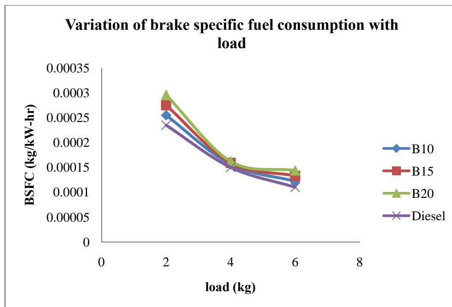
Fig. 2: Variation in brake specific fuel consumption with change in load.
