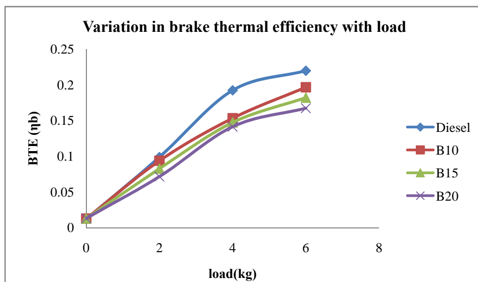
Fig. 3: Variation in brake thermal efficiency with change in load.
