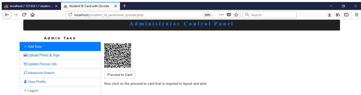
Figure 7: Qrcode Generated
