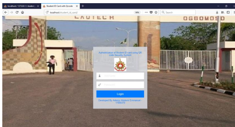
Figure 3: Home Page.
