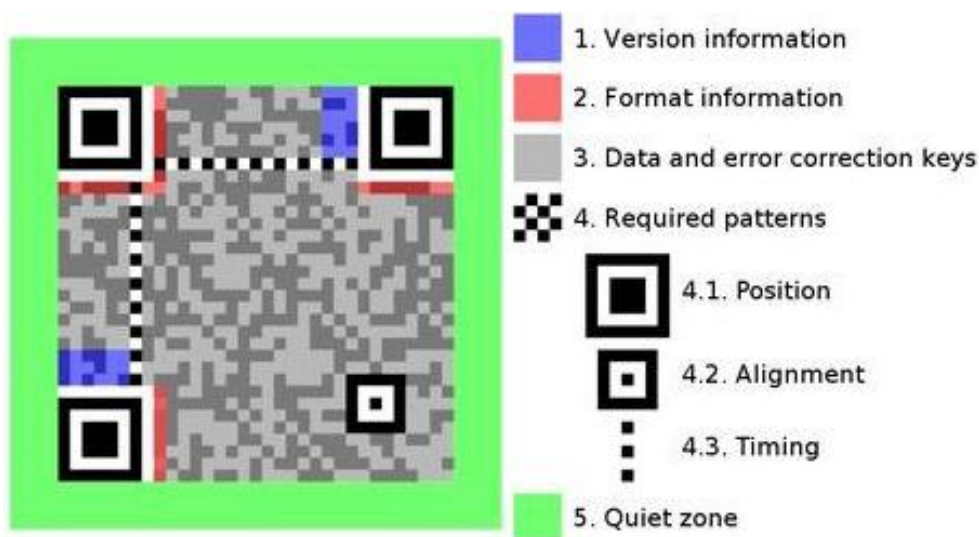
Figure 1: The Structure of Quick Response Code (Ayeleso, et al., 2017)
