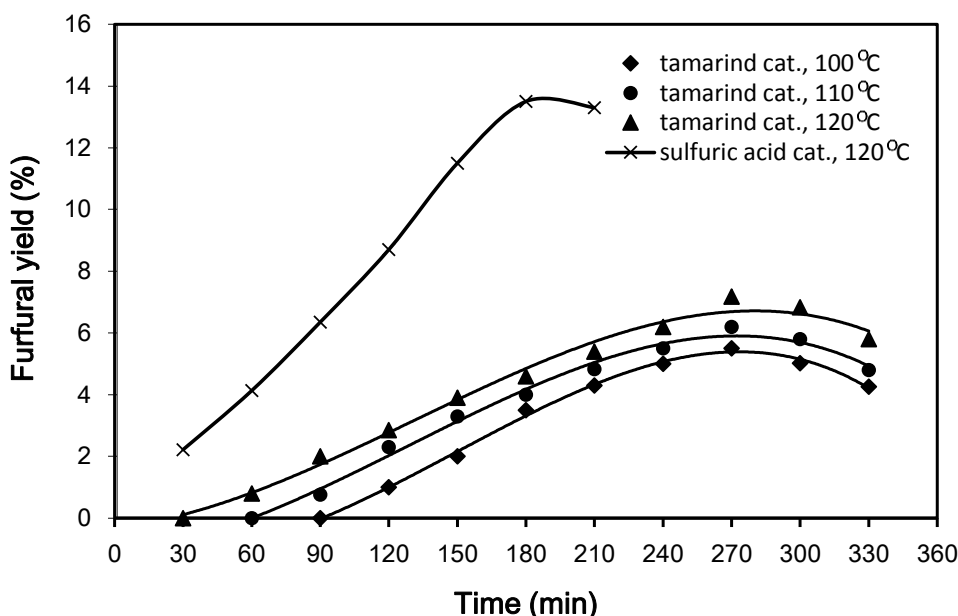
Fig 2. The effect of reaction time on furfural yield at various temperatures
