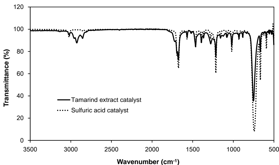
Fig 3. FTIR analysis using tamarind extract and sulfuric acid catalyst
