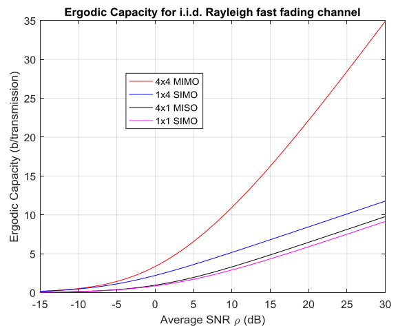
Fig. 10. Relationship between capacity and average SNR
