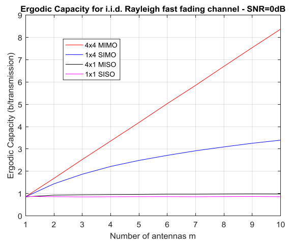
Fig. 9. Capacity vs. number of antennas for a 1 \times 1 SISO system, a 1 \times 4 SIMO system, a 4 \times 1 MISO system, and a 4 \times 4 MIMO system (SNR=0)
