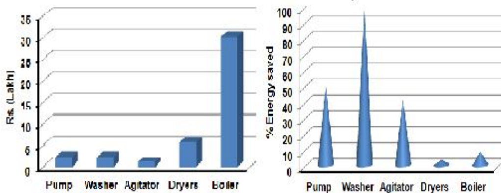
Fig. 1: Cost and Energy saving for the audited sections.
