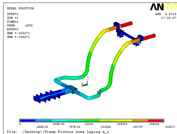
Image 3: Ansys Solution Image
