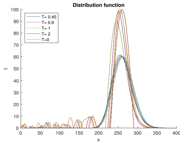
Figure 3: distribution function.
