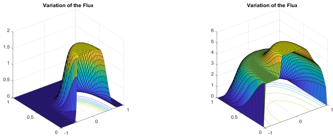
Figure 2: Schrödinger's equation solution at various times.
