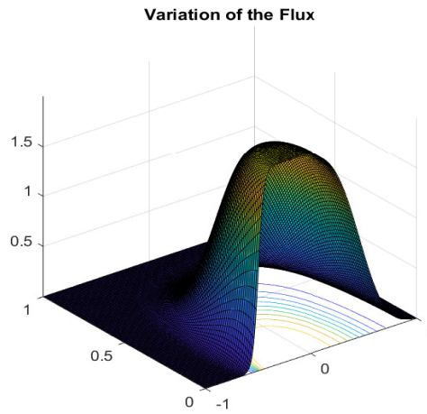
Figure 1: Time evolution of the numerical solution
